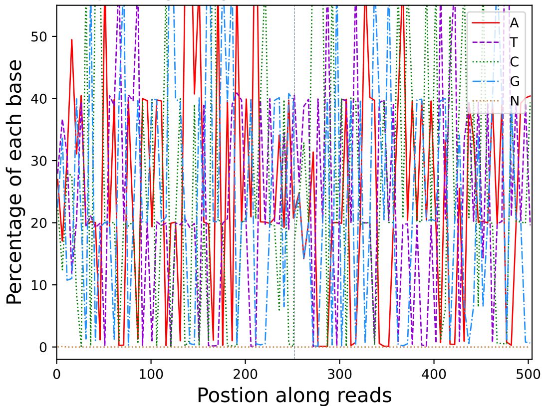
Base percentage along reads (R10628)
